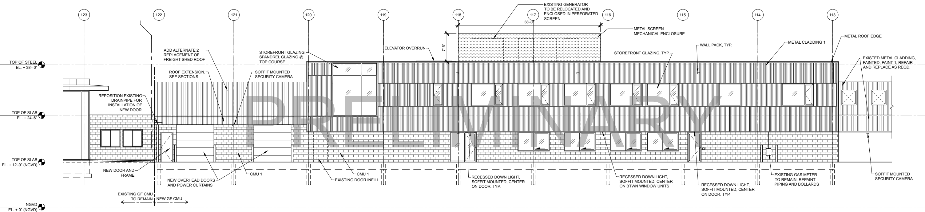
North Elevation
